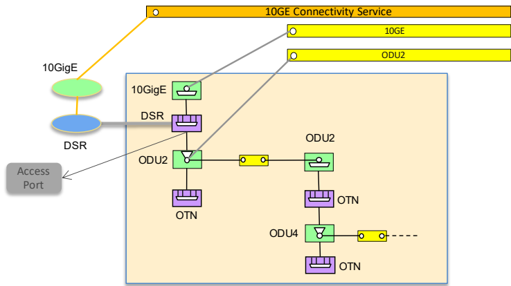
Figure 5-53 Option: No DSR cross-connection, with ODU-LO cross-connection
