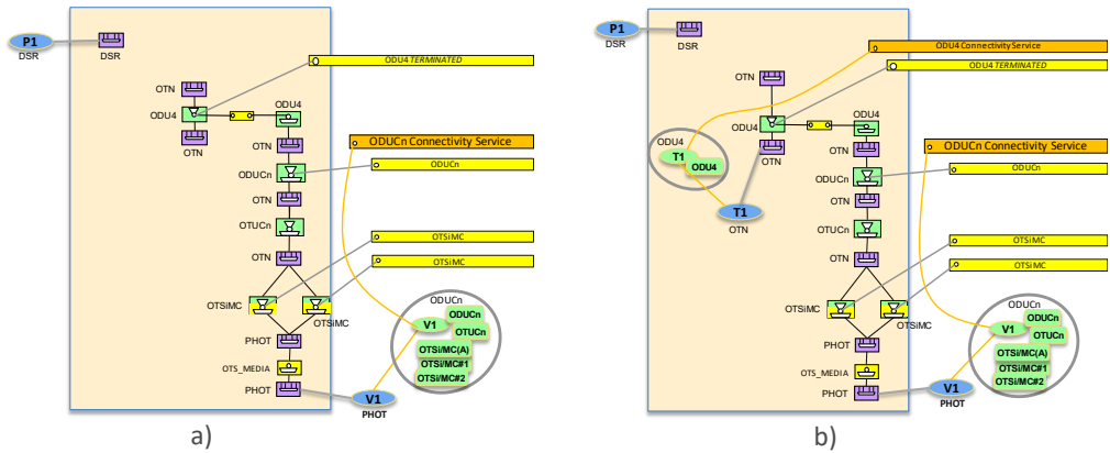
Figure 6-65 a) No server connections, b) Server ODUCh Connectivity Service
