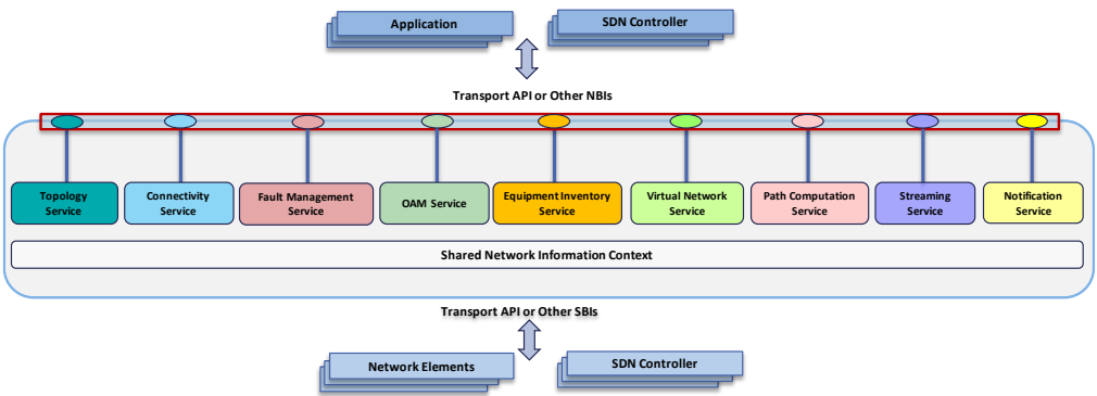
Figure 3-1 Transport API Functional Architecture
