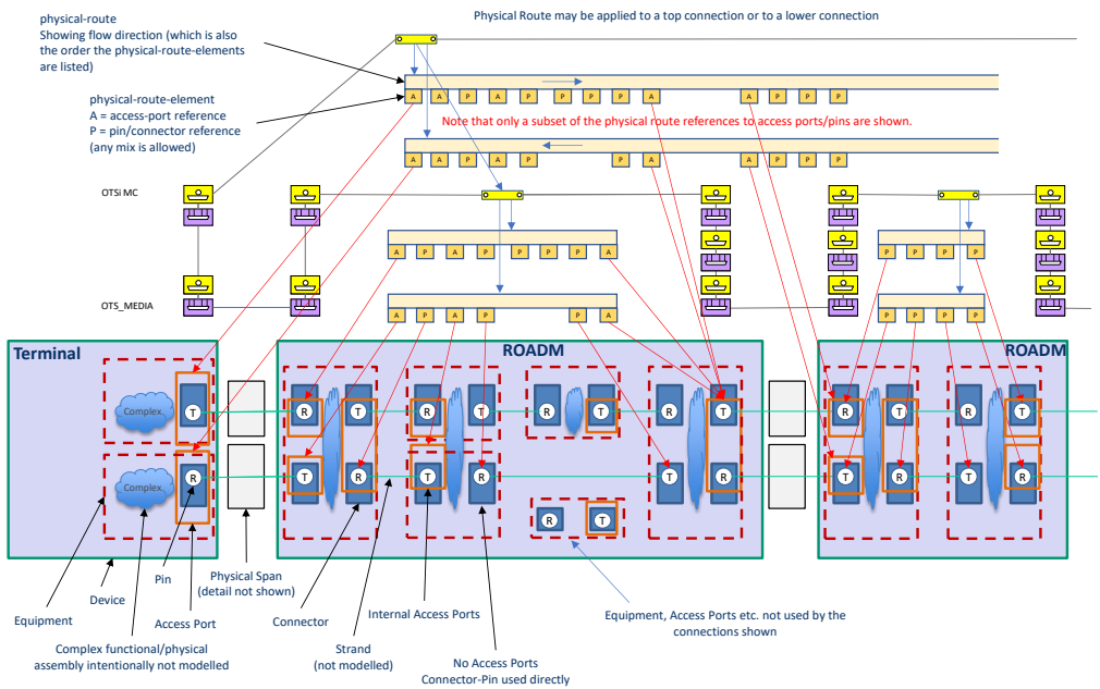
Figure 3-4 View of the Physical Route model
