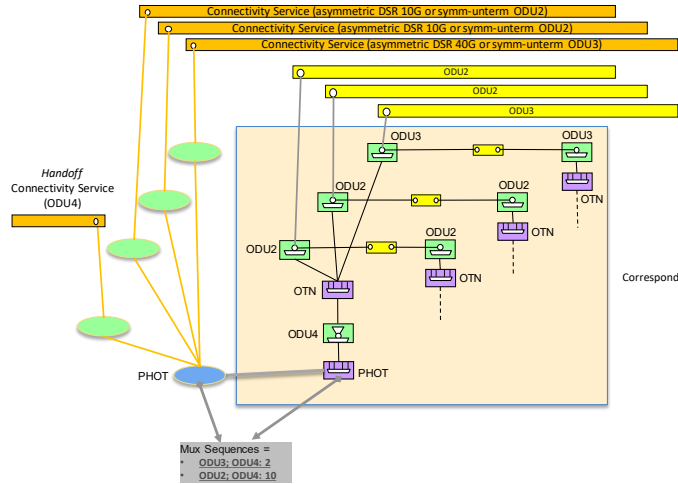
Figure 5-64 OTN ENNI, mapped & multiplexed client protocols
