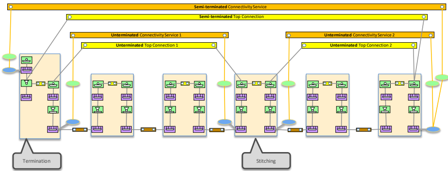
Figure 5-5 Underminated Connection, semi-terminated CS and Connection
