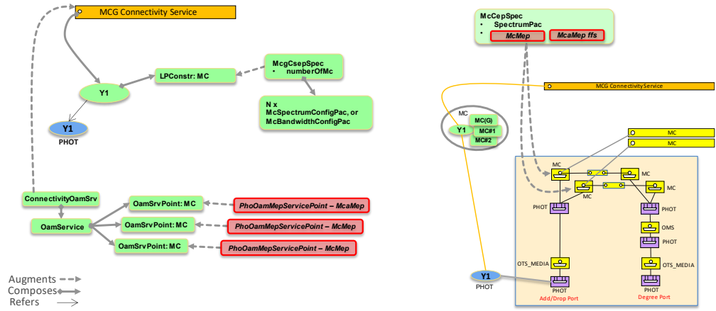
Figure 6-43 MCG Connectivity Service at Add/Drop side
