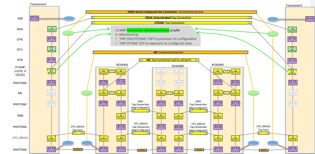
Figure 6-119 Transceiver Profile, configuration and state
