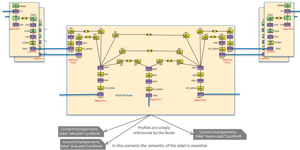
Figure 6-125 Connectivity Impairments – No Node Rule Group
