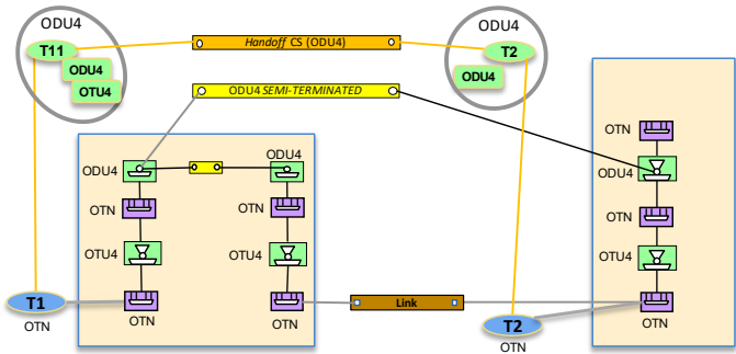
Figure 6-75 Server ODU Handoff Connectivity Service
