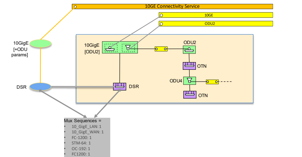
Figure 5-55 Option: Simplified DSR UNI
