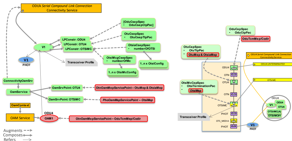
Figure 6-8 ODUk Serial Compound Link Connection Connectivity Service
