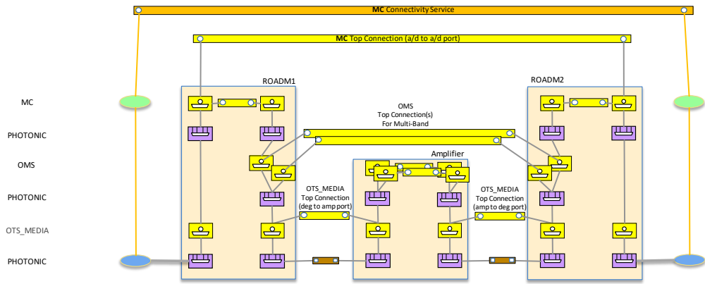
Figure 5-29 Scenario 1 : Optical Line System Controller, multi-band (note: not all MC NEPs are represented)
