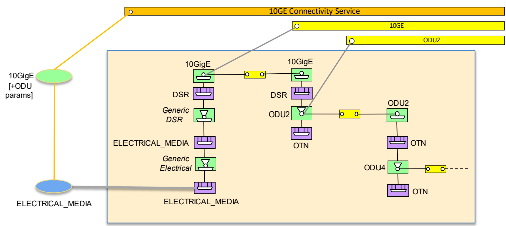
Figure 5-58 DSR UNI, explicit model of functions (electrical)
