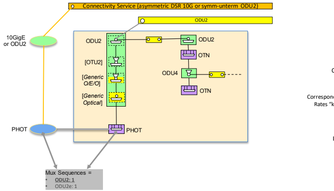
Figure 5-63 OTN ENNI, directly mapped client protocols, with additional embedded functions, 10GE/ODU2
