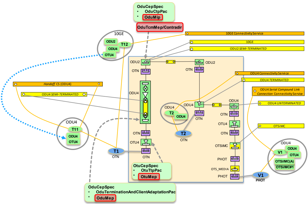
Figure 6-32 Asymmetric scenario 4: DSR/ODUj CS (OTN ENNI) - Explicit ODU4 Handoff CS and Connection
