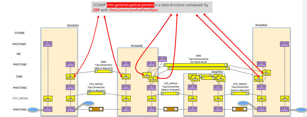
Figure 6-120 OMS Impairments
