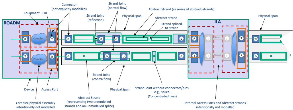
Figure 3-3 View of the Physical Span model
