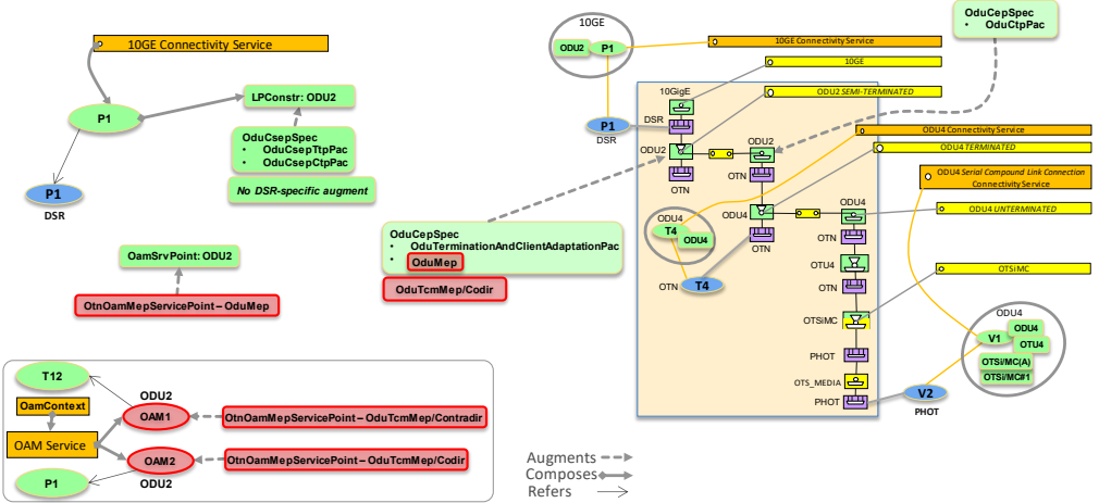
Figure 6-24 Asymmetric scenario 1: DSR/ODUj CS (DSR UNI)
