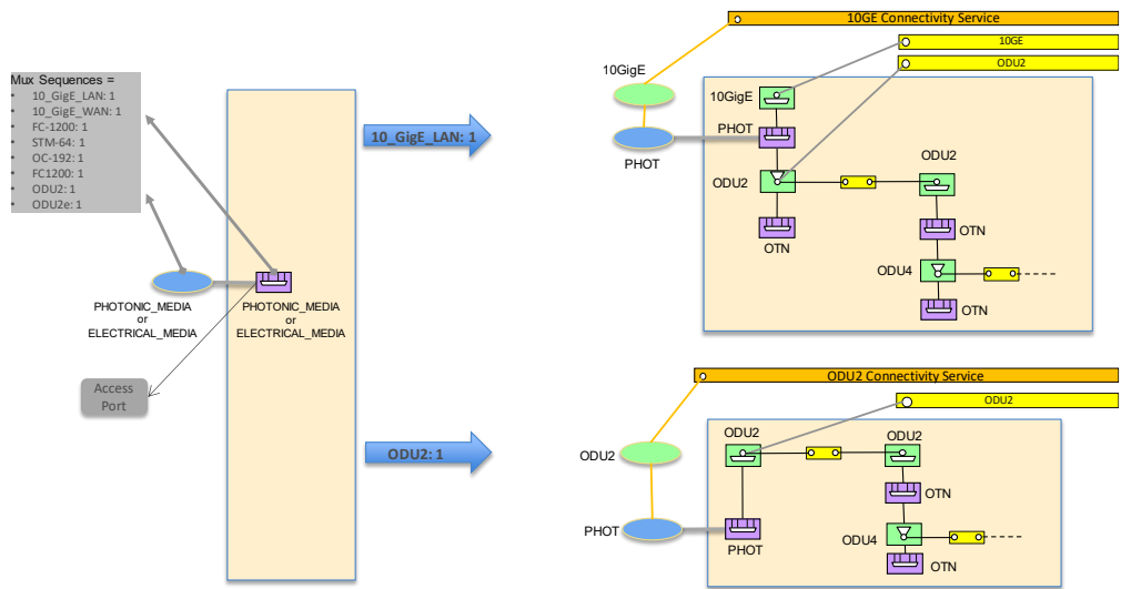
Figure 5-73 DSR/OTN NI, multi-technology interface
