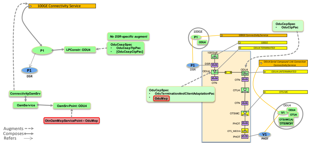
Figure 6-9 DSR/ODUk Connectivity Service on ODUk SCLC CS
