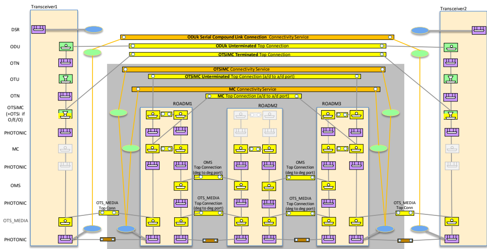
Figure 5-39 Scenario 2 : Integrated Mng, MC CS, unterminted OTSiMC CS, terminated OTSiMC +ODU CSs
