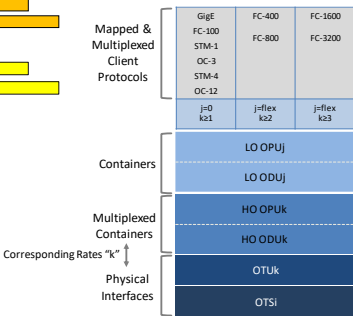
MEF 64 Figure 6 – OTUk Structure for Mapped & Multiplexed Client Protocols
