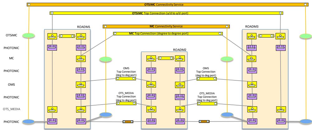
Figure 5-27 Scenario 1 : Optical Line System Controller, OTSiMC and MC CSs
