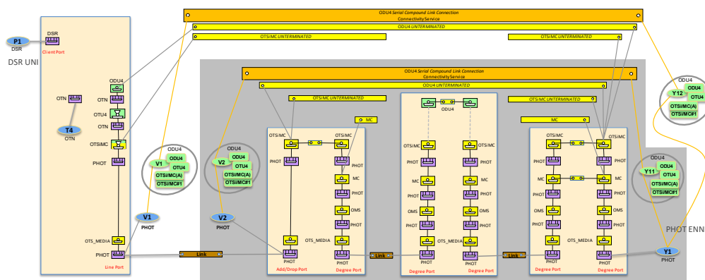
Figure 6-56 ODU Asymmetric scenario with ODU CS in the OLS subnetwork, with 3R
