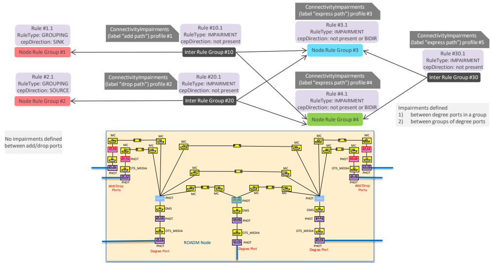
Figure 6-129 Conn. Impairments specified per add , drop and express conns, not homogeneous between express
