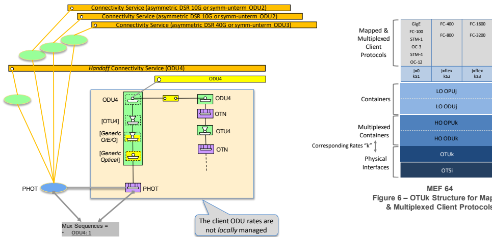
Figure 5-70 OTN ENNI, not locally mapped & multiplexed client protocols, with additional embedded functions
