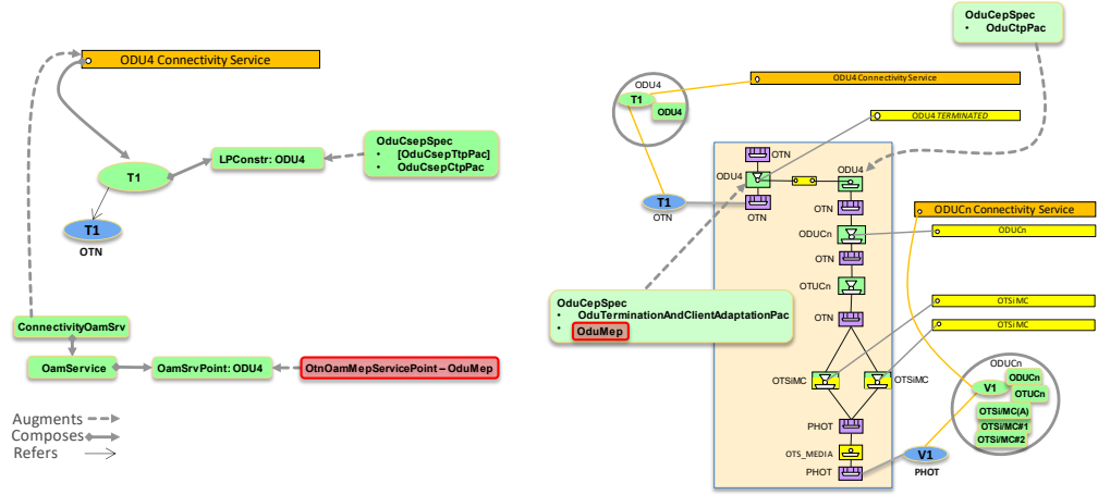
Figure 6-37 Infrastructure or Handoff ODUk CS on ODUcn CS
