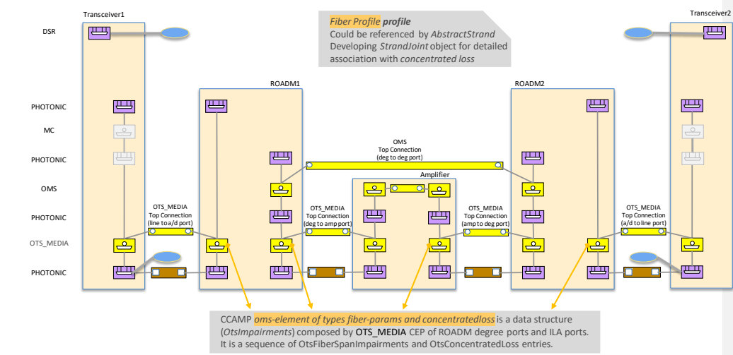
Figure 6-121 OTS Impairments
