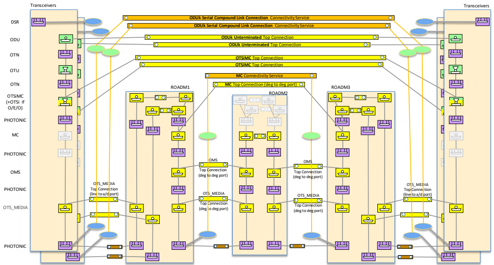
Figure 5-46Figure 5-46 is a variation of the previous scenarios where it is shown multiple add/drop port tributary signals being forwarded to a common express media channel.
