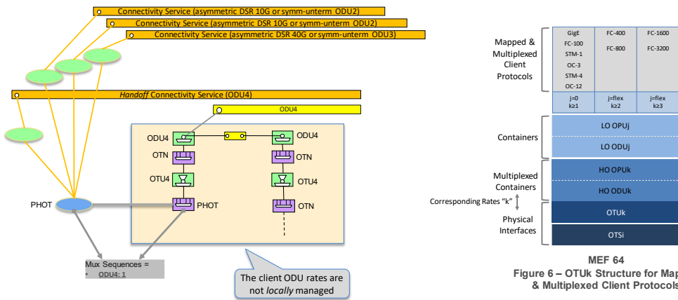
Figure 5-69 OTN ENNI, not locally mapped & multiplexed client protocols, with OTU CEP
