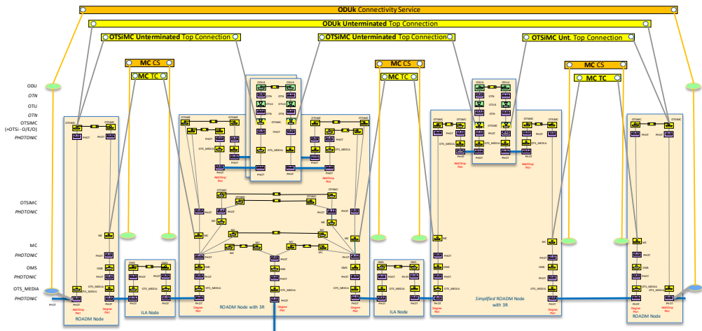
Figure 5-32 Scenario 1 : Optical Line System Controller, regeneration
