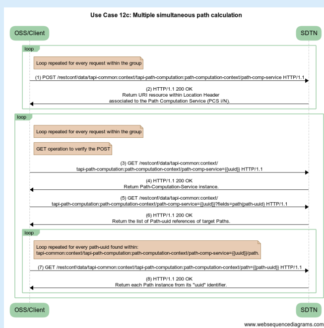
Figure 7 18 UC-12c: Multiple simultaneous path computation
