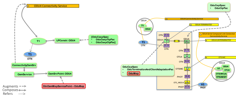
Figure 6-14 Infrastructure or Handoff ODUk Connectivity Service on ODUk SCLC CS
