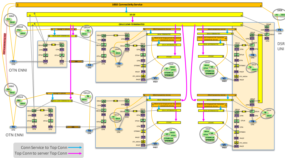
Figure 5-18 - Asymmetric ODU2 SNCP - Relationships between CSs and Top Connections
