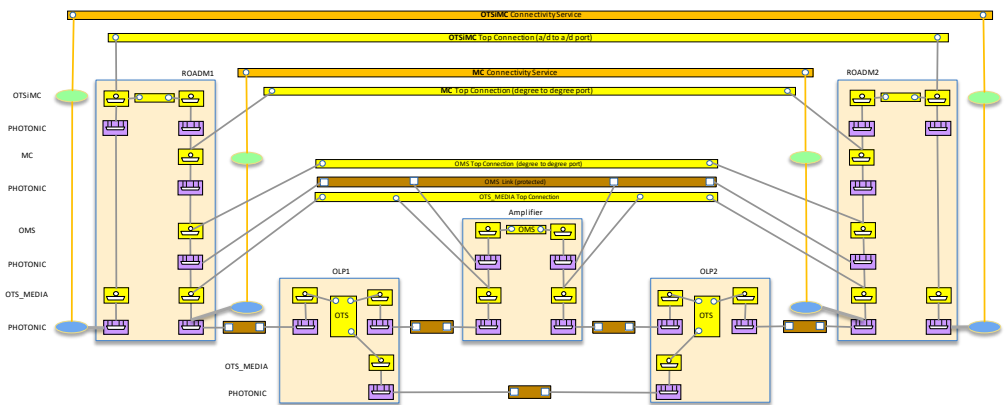
Figure 6-84 UC-5a OLP protection TAPI representation 1
