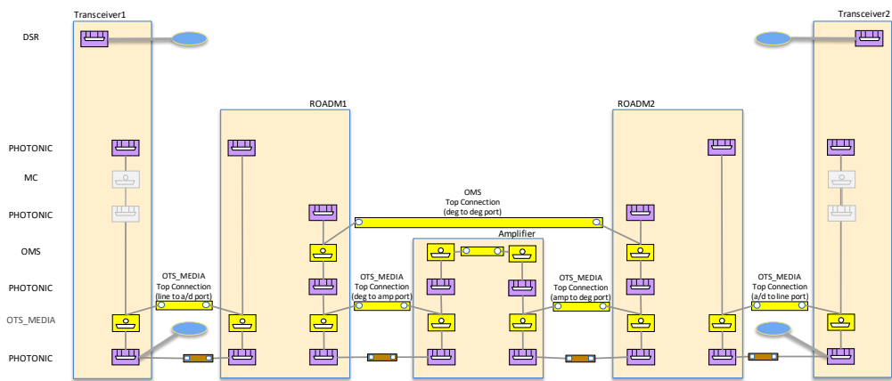
Figure 5-33 Scenario 2 : Integrated Management, time zero
