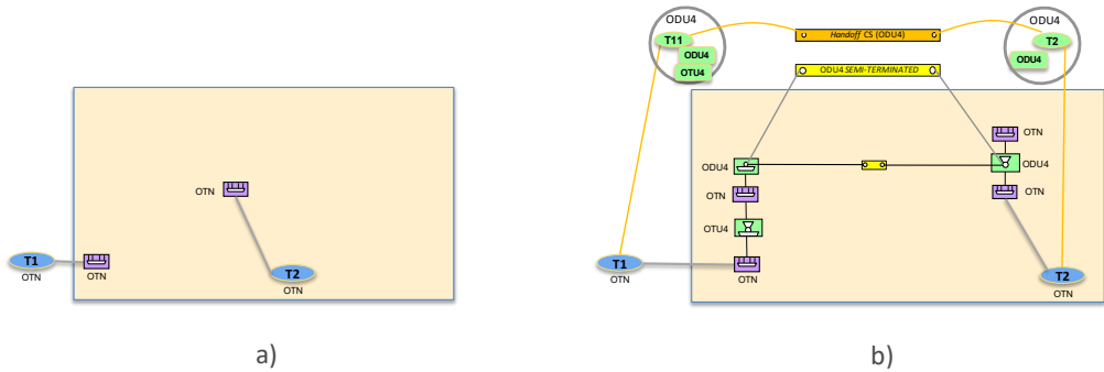
Figure 6-78 a) No "server" connections, b) Server ODU Handoff Connectivity Service
