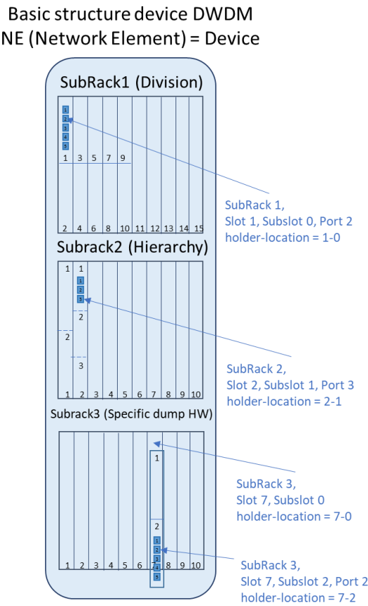
Figure 6-83 UC-4b Network Element Subracks container-holder location examples.
