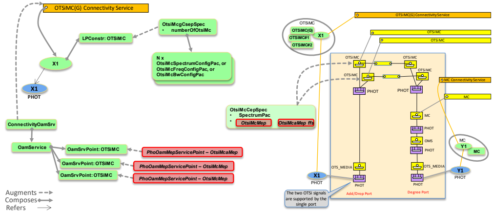
Figure 6-53 shows the configuration parameters for the provisioning of the OTSiMC(G) connectivity service on an existing MC Connectivity Service. The result includes the OTSiMC connection(s) which support the OTSiMC(G).
