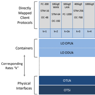
MEF 64 Figure 5 – OTUk Structure for Directly Mapped Client Protocols
