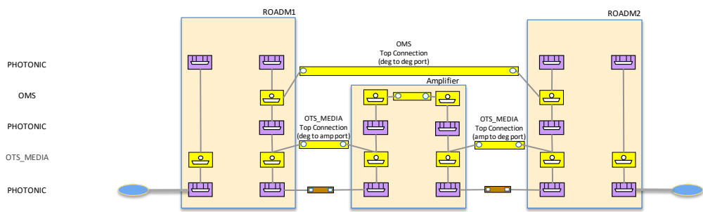
Figure 5-22 Scenario 1 : Optical Line System Controller, time zero, In Line Amplifier
