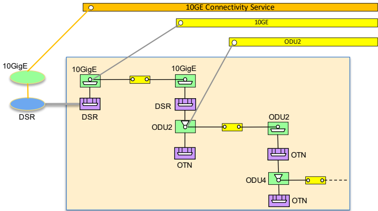
Figure 5-51 Option: Explicit DSR cross-connection
