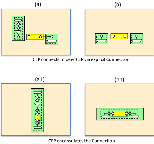
Figure 5-2 Explicit and encapsulated connections
