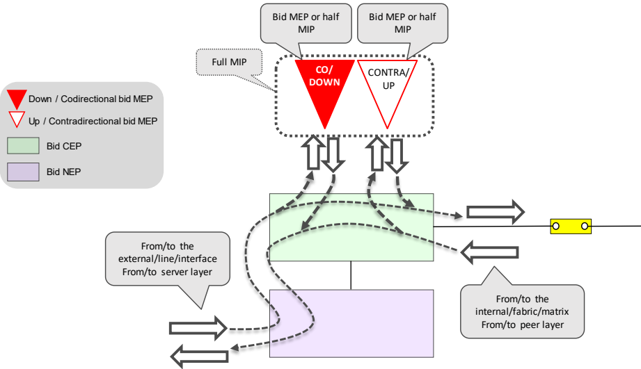
Figure 5-16 Bidirectional CEP, MEP, and MIP monitoring orientation
