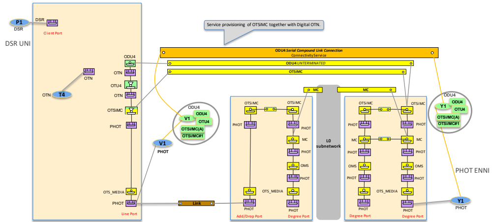
Figure 5-78 PHOTONIC ENNI, integrated scenario, without 3R
