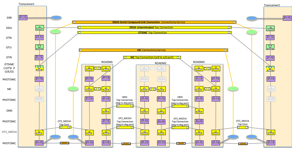
Figure 5-36 Scenario 2 : Integrated Management, MC and OTSiMC+ODU CSs
