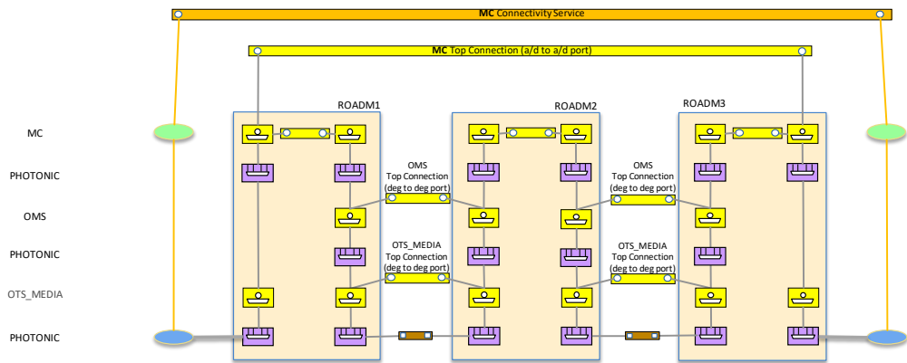
Figure 5-23 Scenario 1 : Optical Line System Controller, MC CS
