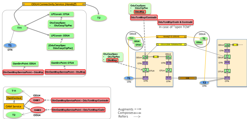
Figure 6-21 Asymmetric scenario 1: ODUk Handoff CS (OTN ENNI) – Part 1
