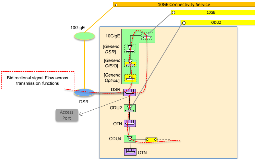
Figure 5-57 Option: DSR UNI with additional embedded functions with explicit DSR and ODU cross-connections (top), simplified without DSR cross-connection (middle), and simplified without cross-connections (bottom)
