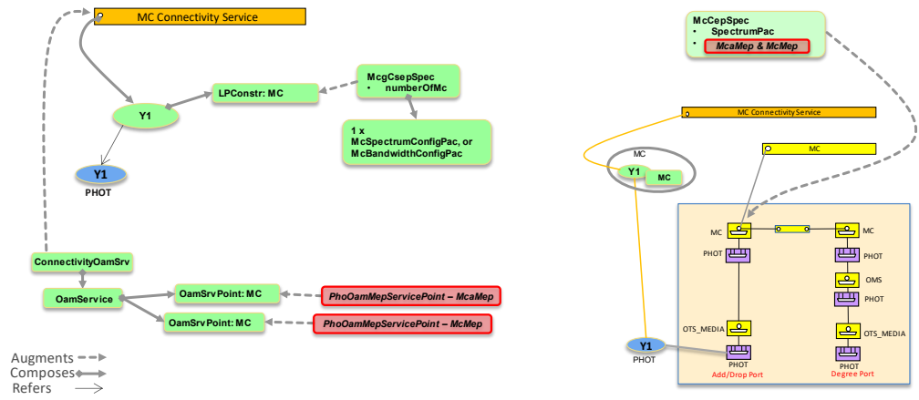
Figure 6-42 MC Connectivity Service at Add/Drop side
