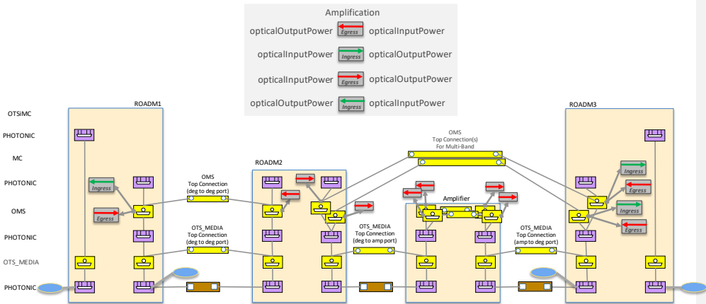
Figure 6-122 Amplification Impairments
