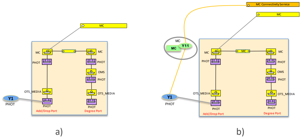
Figure 6-71 a) "Server" MC Connection, b) "Server" MC Connectivity Service
