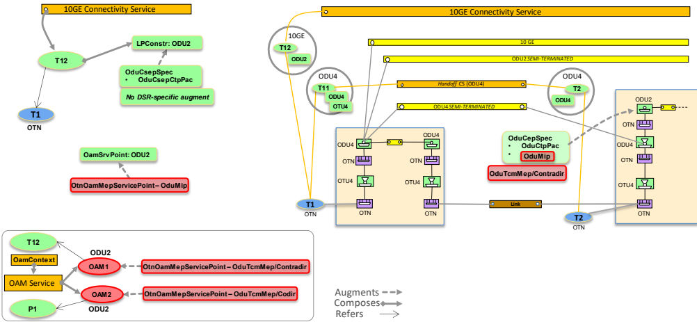
Figure 6-23 Asymmetric scenario 1: DSR/ODUj CS (OTN ENNI)
