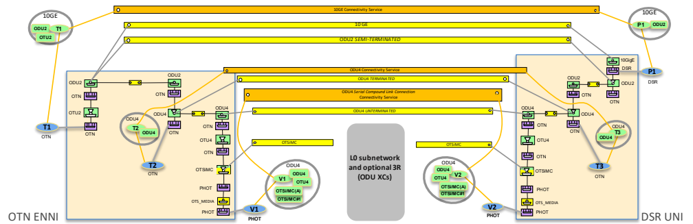
Figure 6-19 Asymmetric Scenario 3: Handoff at ODU2 Layer
