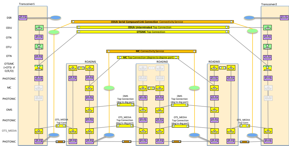
Figure 5-44 Scenario 2 : Integrated Management, MC and OTSiMC+ODU CSs
