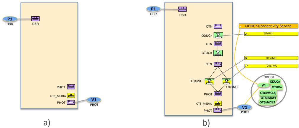
Figure 6-65 a) No server connections, b) Server ODUCh Connectivity Service
