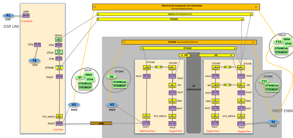
Figure 5-75 PHOTONIC ENNI, no 3R
