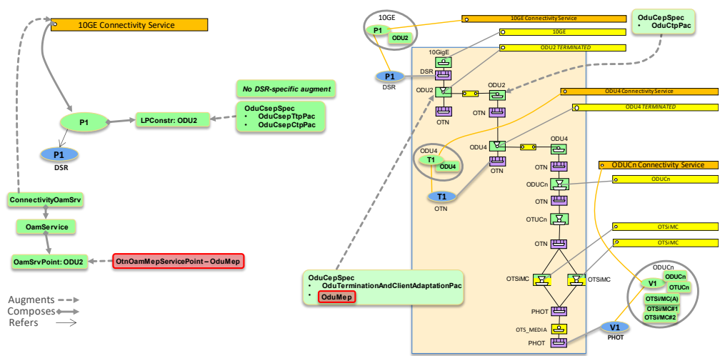
Figure 6-38 DSR/ODUj CS on ODUk CS on ODUCn CS
