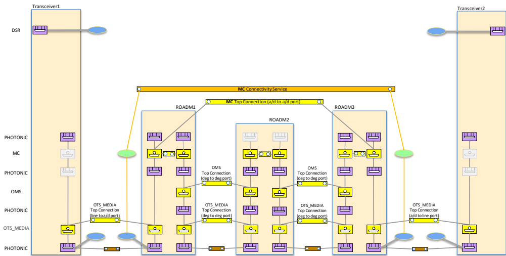
Figure 5-35 Scenario 2 : Integrated Management, MC CS
