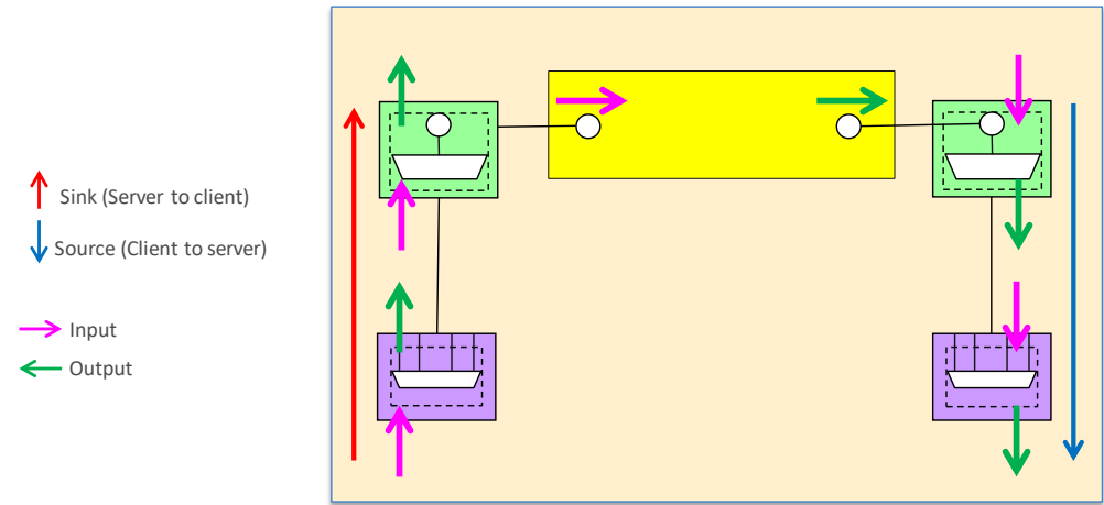
Figure 5-7 Interpreting the direction attributes – non terminated CEPs
