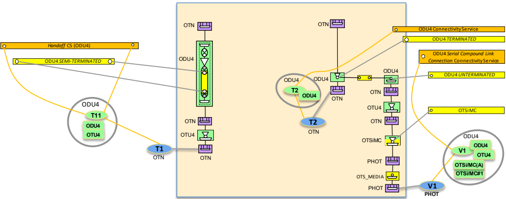
Figure 6-80 Server ODU Handoff Connectivity Service
