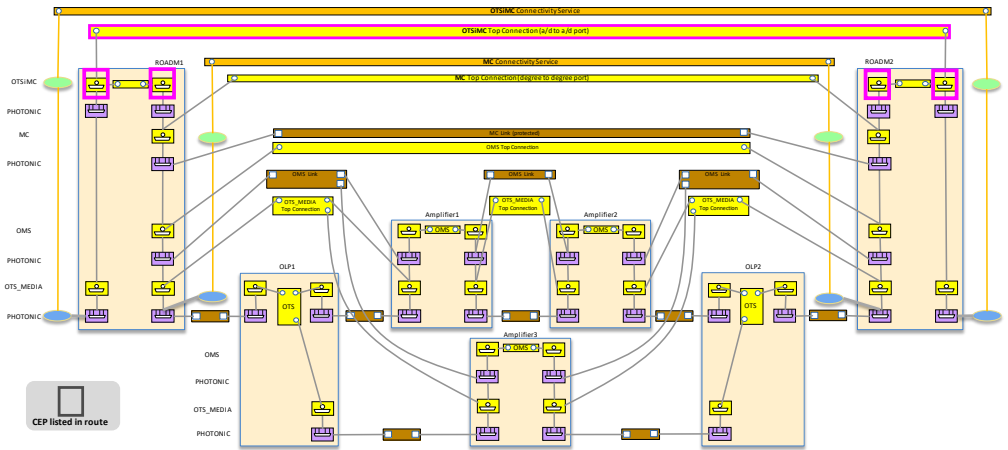
Figure 6-95 UC-5a OLP protection TAPI representation 3, OTSiMC route
