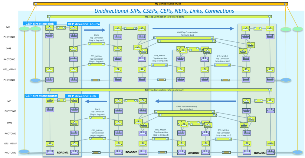
Figure 6-70 Full Unidirectional - UNI and OMS unidirectional scenario.
