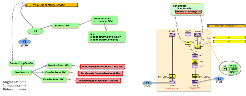
Figure 6-49 MCG Connectivity Service at Degree side
