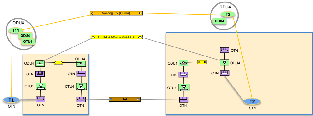
Figure 6-77 Server ODU Handoff Connectivity Service, variation
