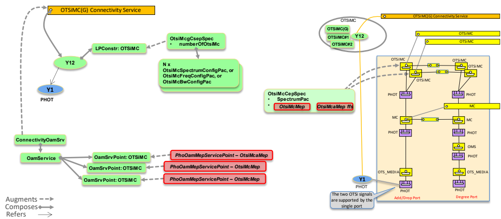
Figure 6-45 OTSiMCG CS on existing MC Connection at Add/Drop side
