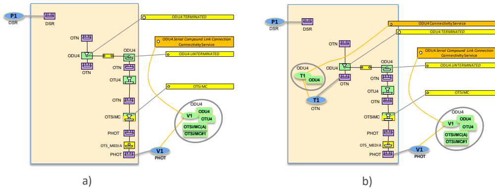
Figure 6-62 a) No server connections, b) Server ODU SCLC Connectivity Service
