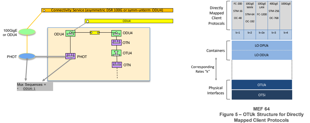
Figure 5-60 OTN ENNI, directly mapped client protocols
