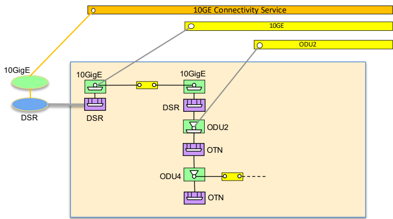
Figure 5-52 Option: Explicit DSR cross-connection, no ODU-LO cross-connection
