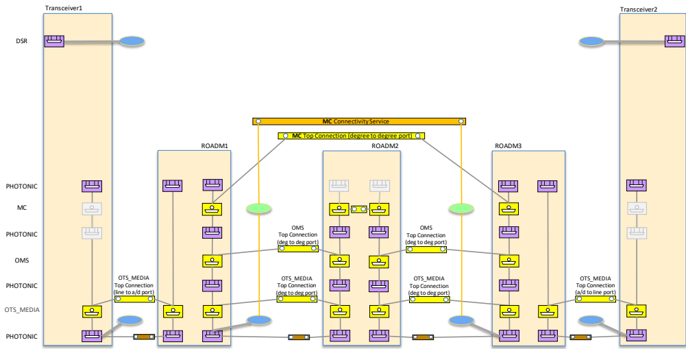
Figure 5-43 Scenario 2 : Integrated Management, MC CS
