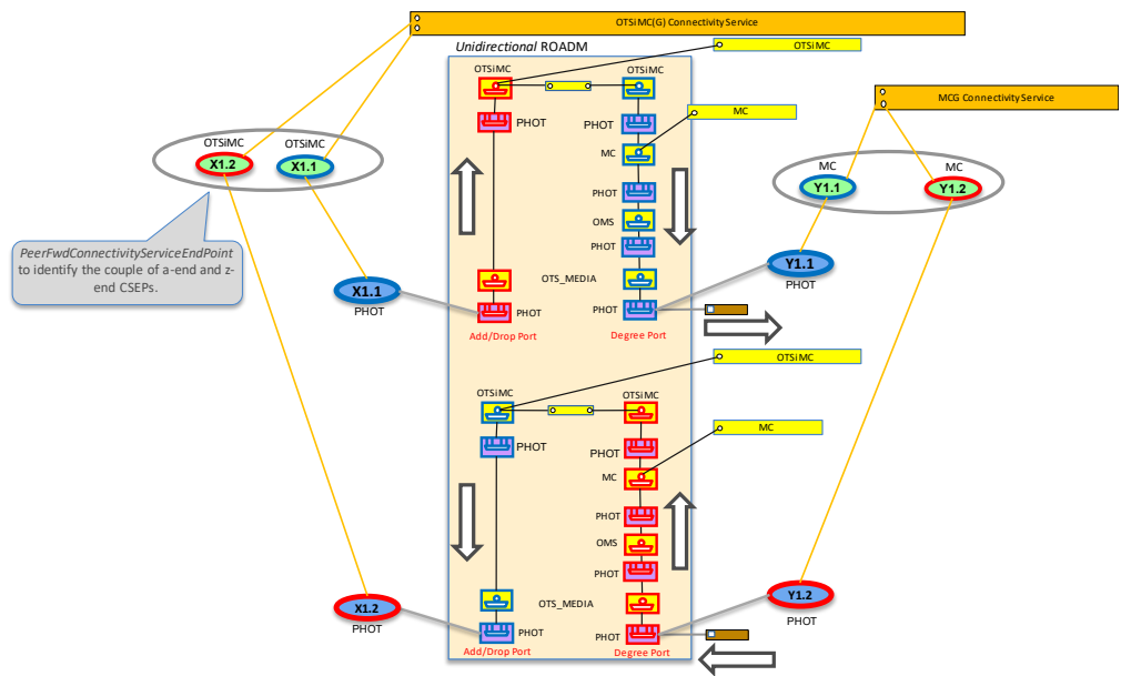
Figure 5-14 OTSiMC with unidirectional CSEPs, second case
