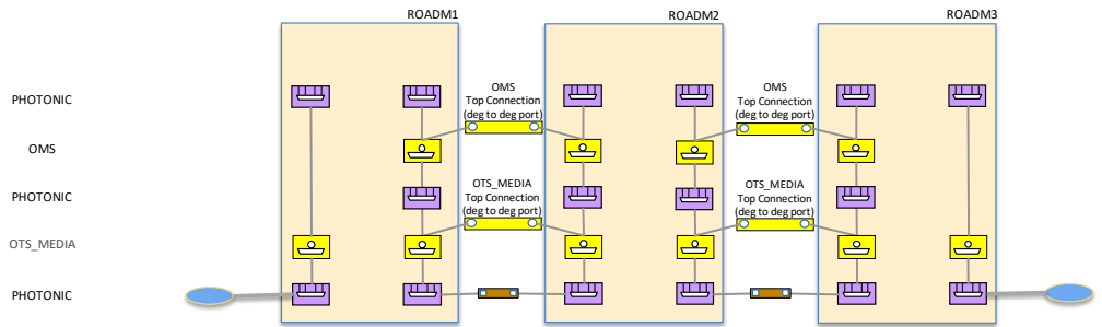
Figure 5-21 Scenario 1 : Optical Line System Controller, time zero
