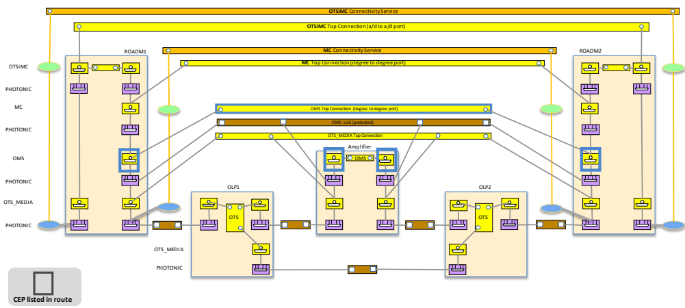
Figure 6-87 UC-5a OLP protection TAPI representation 1 – OMS route
