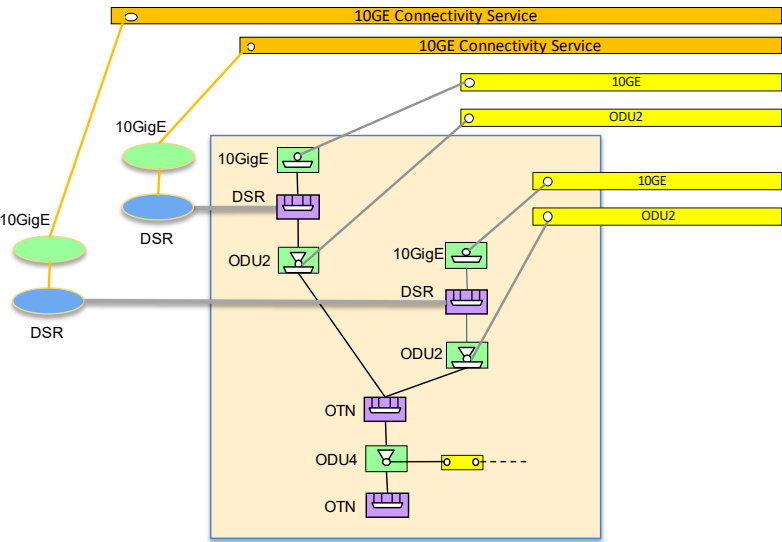
Figure 5-54 Option: No DSR/ODU-LO cross-connections
