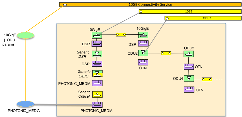
Figure 5-59 DSR UNI, explicit model of functions (optical)
