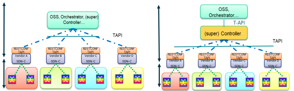
Figure 1-1 Example SDN architecture for WDM/OTN network
