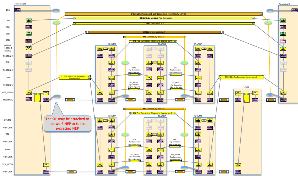
Figure 6-107 UC-5b with embedded OLP within the transponder
