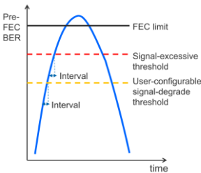
Figure 3-5 FEC function related thresholds
