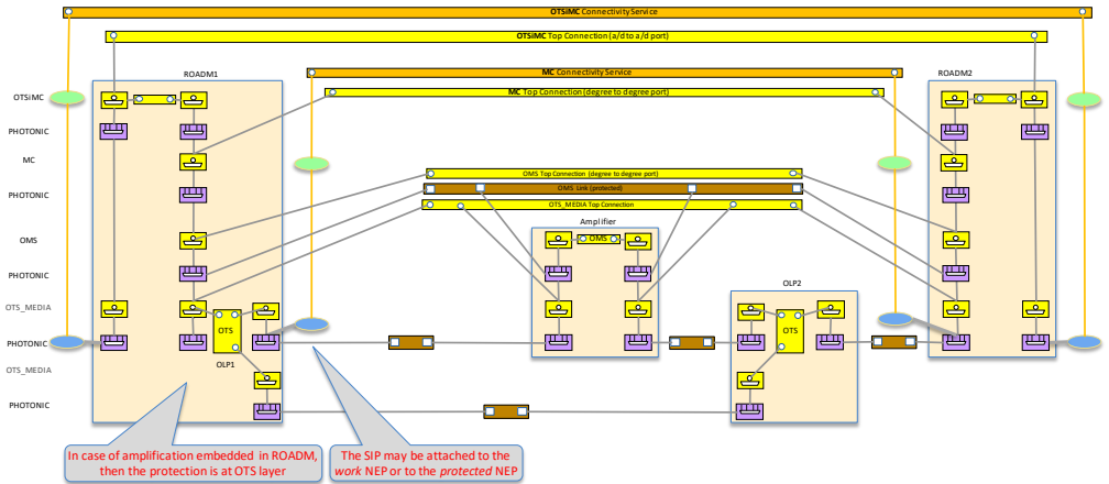
Figure 6-96 UC-5a OLP protection TAPI representation 4, with OLP function embedded in ROADM1
