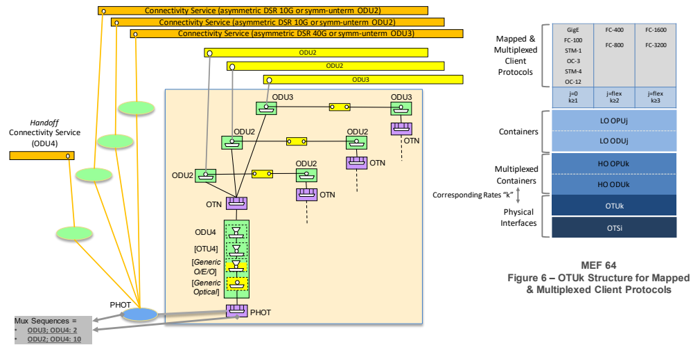
Figure 5-66Figure 5-66 shows the possible embedded transmission functions.
