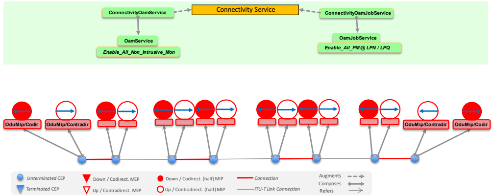
Figure 6-145 OAM provisioning, Server Controller creates/activates NIM OAM parameters of all CEPs
