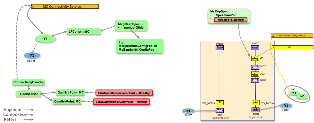
Figure 6-48 MC Connectivity Service at Degree side
