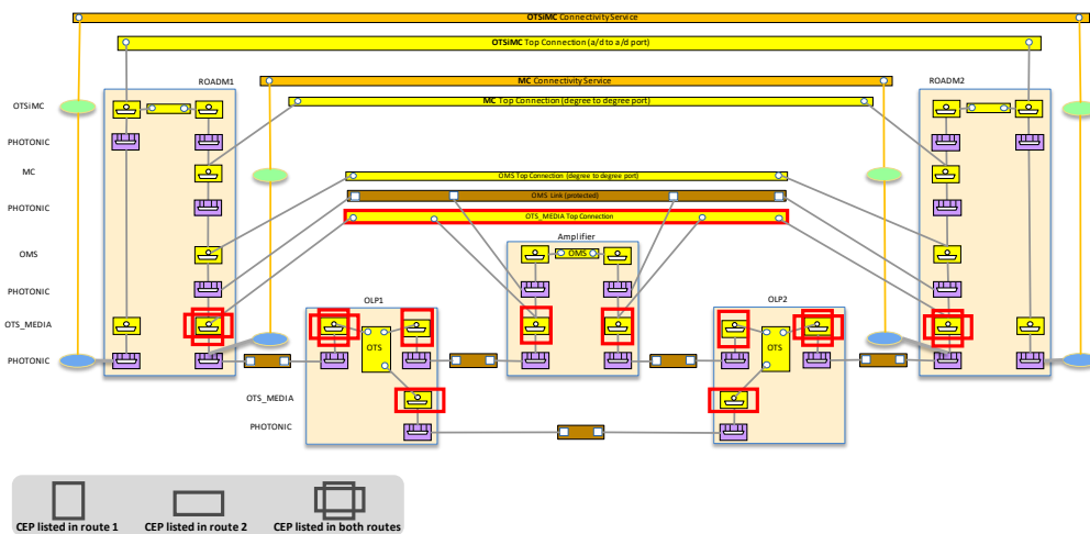
Figure 6-86 UC-5a OLP protection TAPI representation 1 – OTS_MEDIA routes
