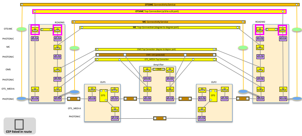
Figure 6-88 UC-5a OLP protection TAPI representation 1 – OTSiMC route
