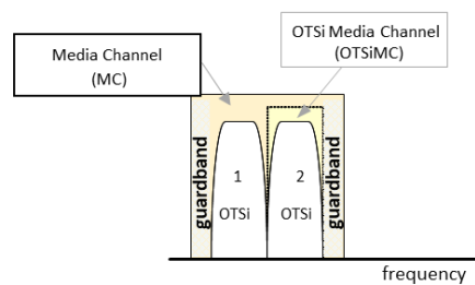
Figure 4-1 Media-channel entities relationship.
