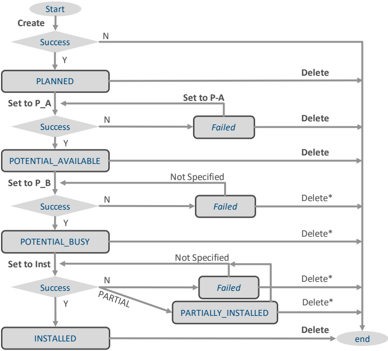
Figure 6-61 Lifecycle state diagram of a connectivity service
