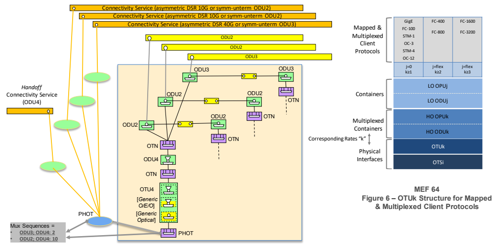
Figure 5-67 OTN ENNI, mapped & multiplexed client protocols, with additional embedded functions of OTU CEP
