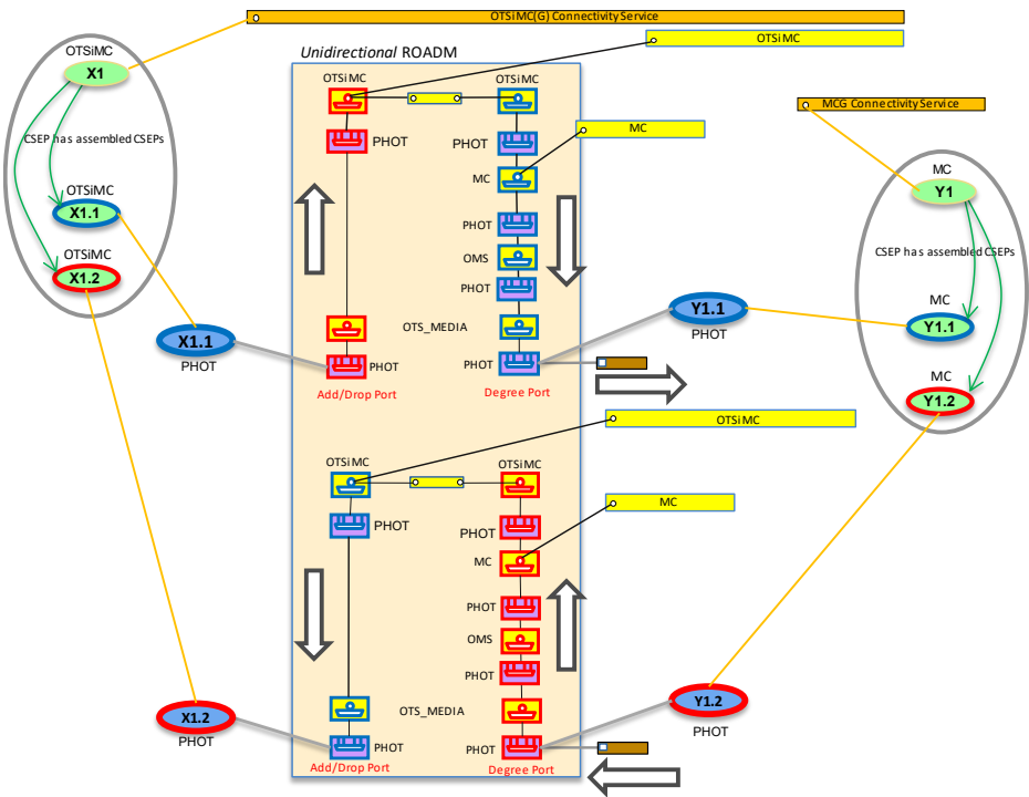
Figure 5-13 OTSiMC with unidirectional CSEPs, first case
