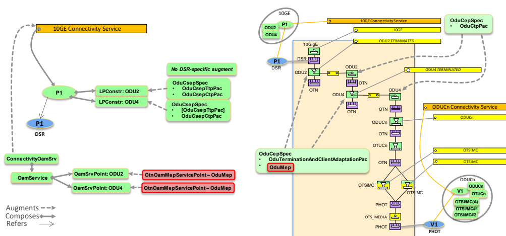
Figure 6-35 DSR/ODUj CS on ODUk on ODUCn CS - ODUk Terminated Connection automatically created or reused
