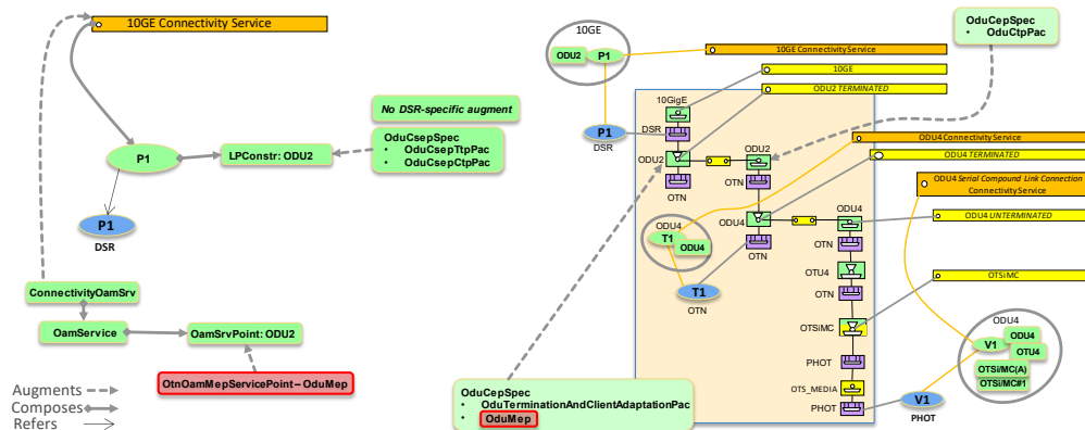
Figure 6-15 DSR/ODUj Connectivity Service on ODUk CS on ODUk SCLC CS
