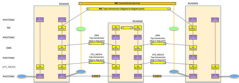
Figure 5-26 Scenario 1 : Optical Line System Controller, MC CS
