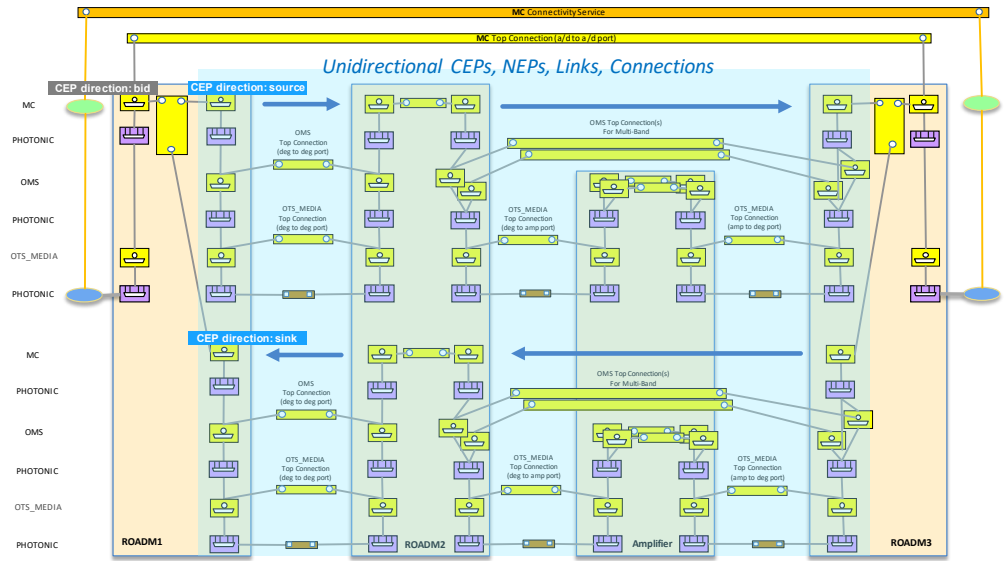
Figure 6-69 Mixed Scenario - UNI bidirectional and OMS unidirectional.
